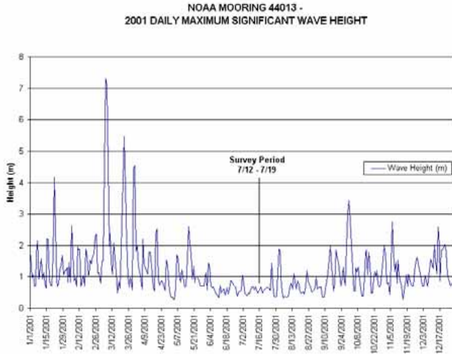
Figure 4.1-1. NOAA Wave Heights
