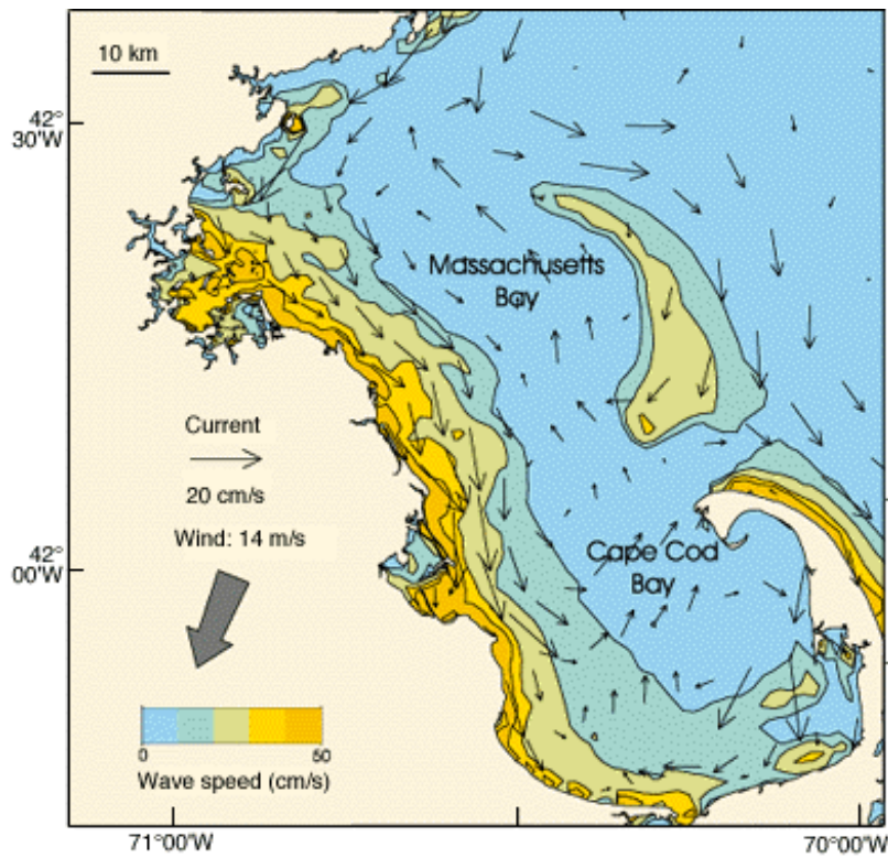
Figure 4.1-2. Contours of near-bottom wave current speed driven by a northeasterly wind of 14 m/s (28 knots) (from USGS Fact Sheet 172-97, February 1998).
