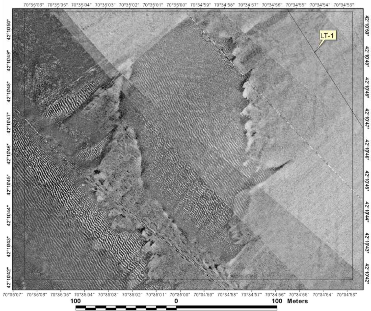
Figure 4.2-2b. Sand Waves at Little Tow
