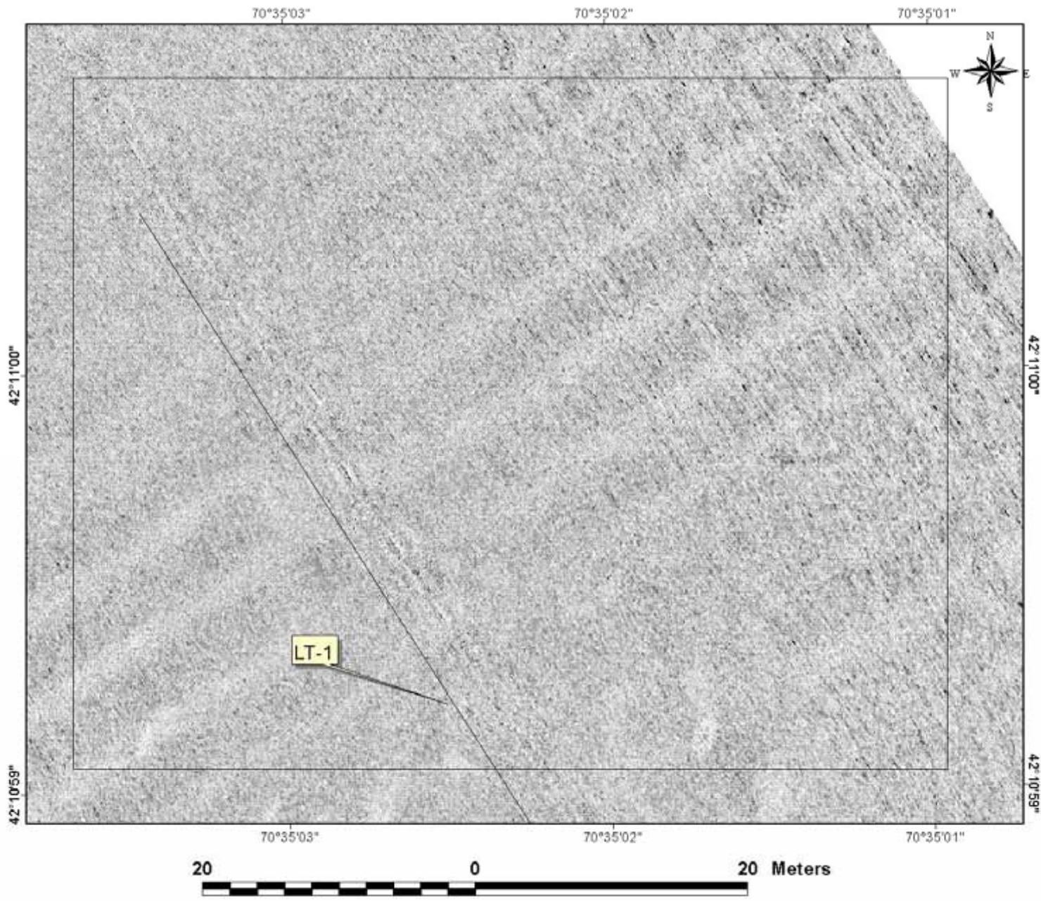
Figure 4.2-2c. Muddy Sand at Little Tow
