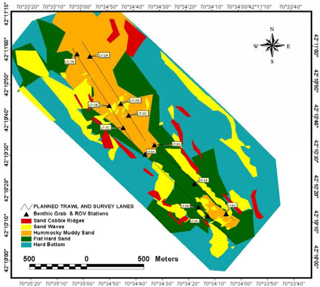
Figure 4.2-4. Bottom Habitat Map of Little Tow
