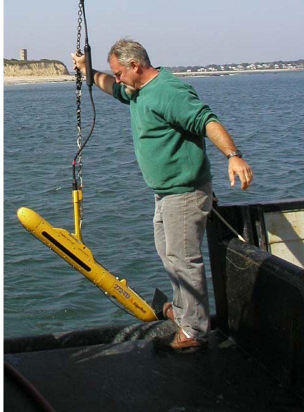
Photograph 3.3-1 Chip Ryther with Edgetech side-scan towfish
